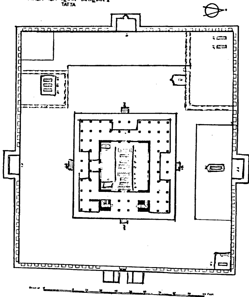
PLAN OF THE TOMB OF MIRZA 'ISA KHAN TARKHAN I TATTA
